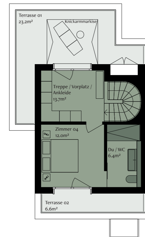
Attika
